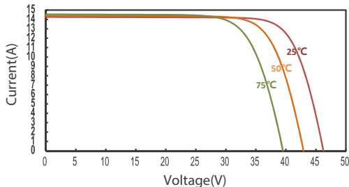
IV Curves of JT475St(B) at different Temp
